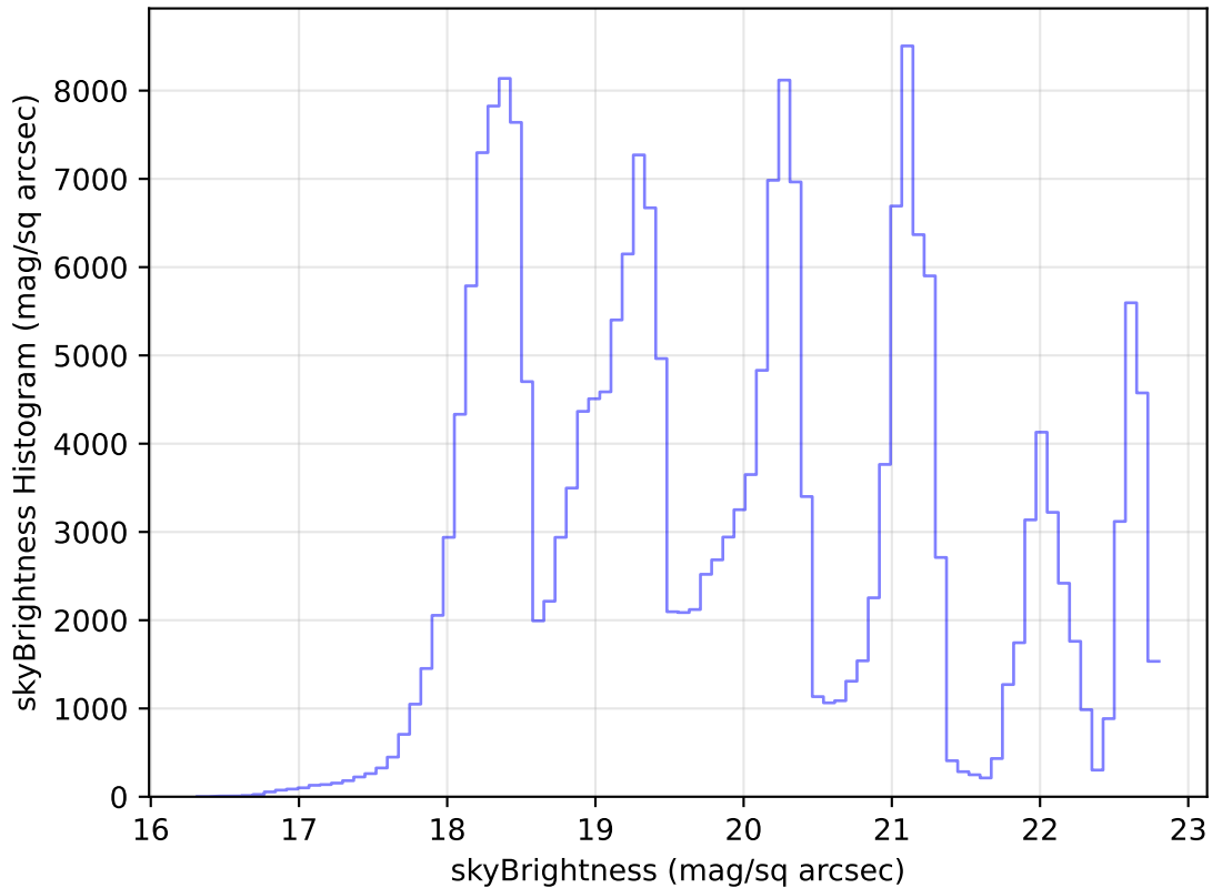
too_elab_r64_d2_griz_v3.4_10yrs Yr 1 all bands: skyBrightness Histogram
