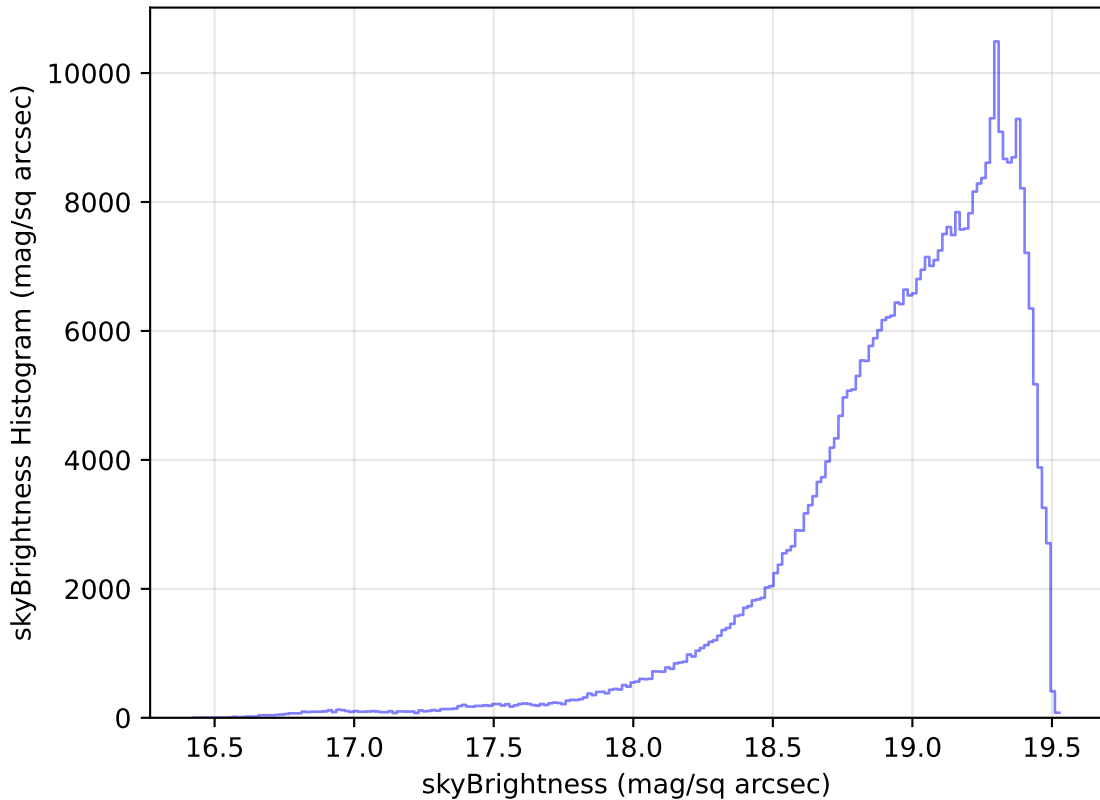
too_elab_r64_d2_griz_v3.4_10yrs WFD z band: skyBrightness Histogram
