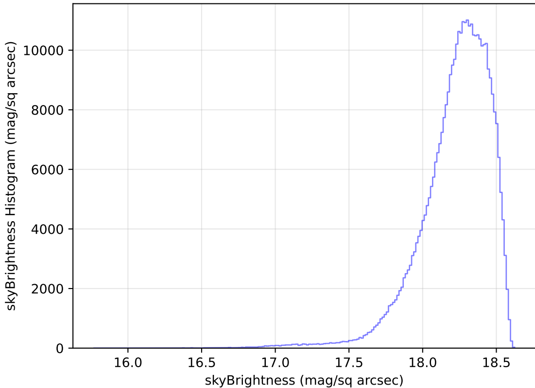
too_elab_r64_d2_griz_v3.4_10yrs WFD y band: skyBrightness Histogram
