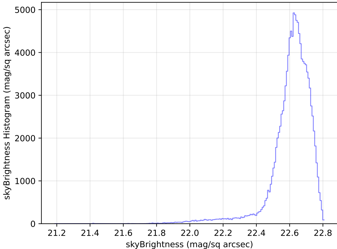
too_elab_r64_d2_griz_v3.4_10yrs WFD u band: skyBrightness Histogram
