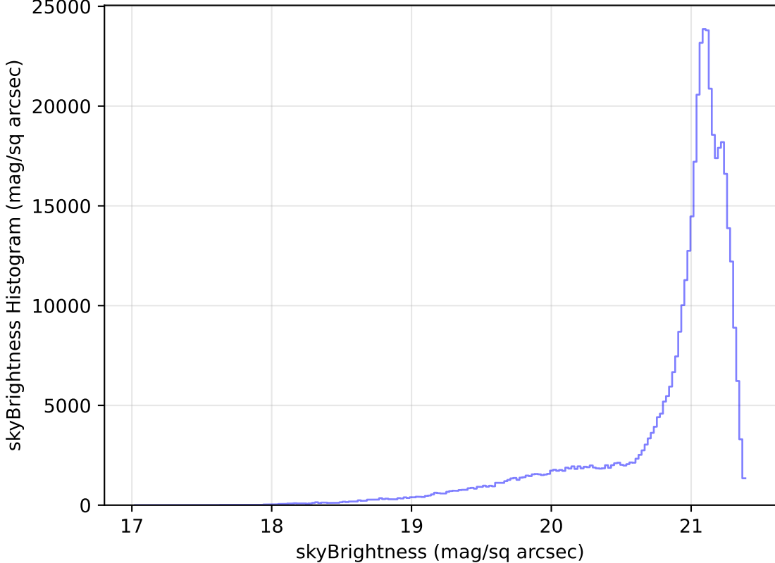
too_elab_r64_d2_griz_v3.4_10yrs WFD r band: skyBrightness Histogram
