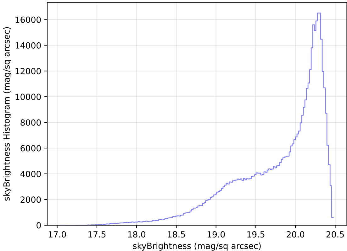
too_elab_r64_d2_griz_v3.4_10yrs WFD i band: skyBrightness Histogram
