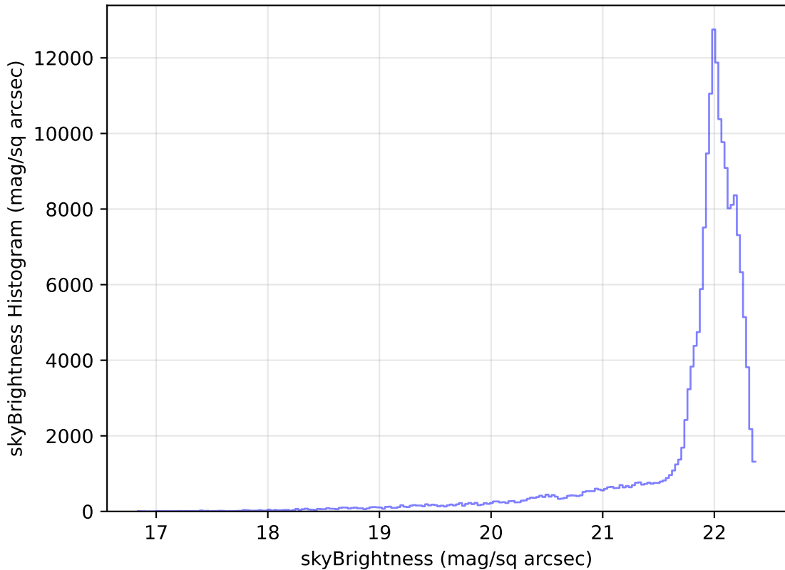
too_elab_r64_d2_griz_v3.4_10yrs WFD g band: skyBrightness Histogram
