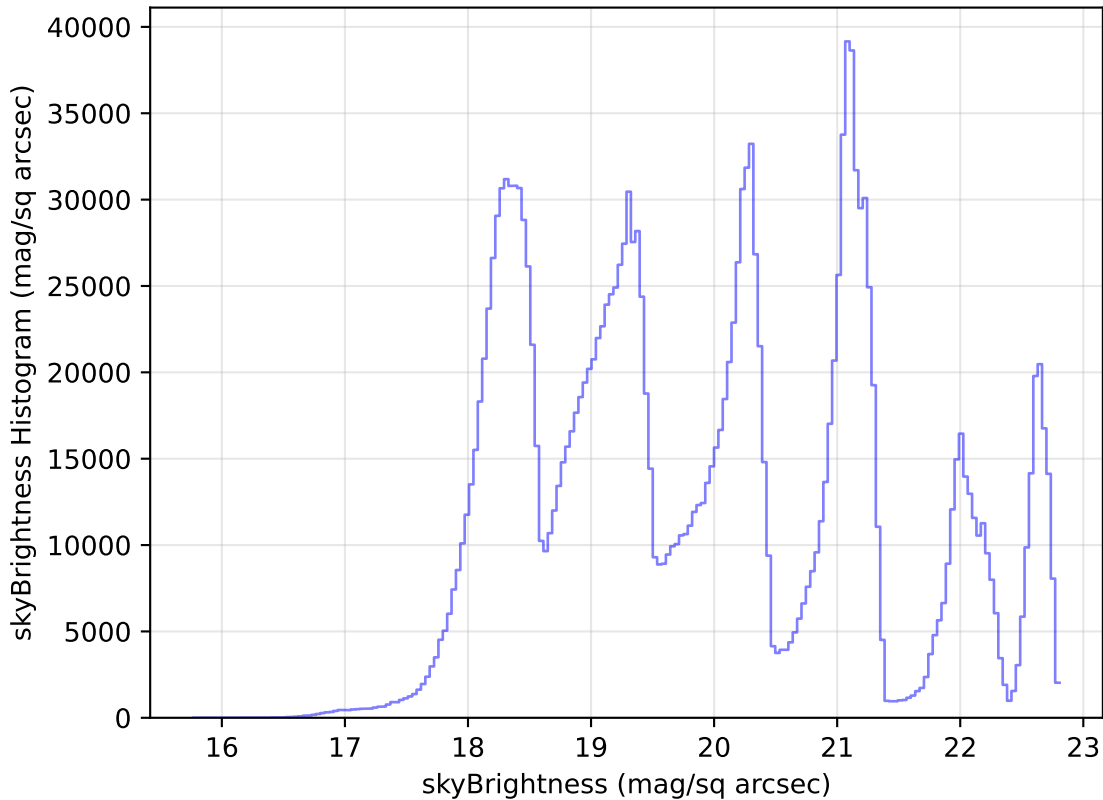
too_elab_r64_d2_griz_v3.4_10yrs WFD all bands: skyBrightness Histogram
