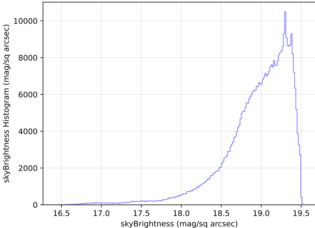
too_elab_r64_d2_griz_v3.4_10yrs All sky z band: skyBrightness Histogram
