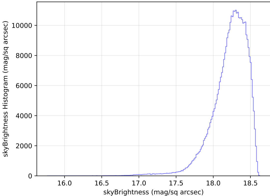
too_elab_r64_d2_griz_v3.4_10yrs All sky y band: skyBrightness Histogram
