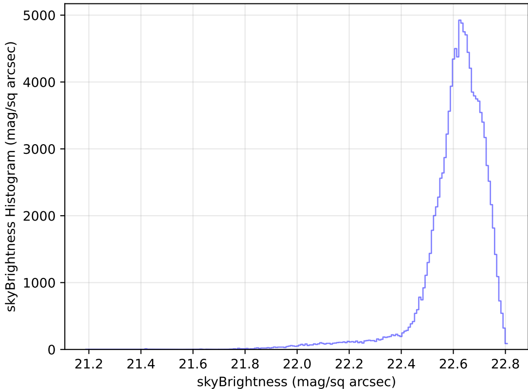
too_elab_r64_d2_griz_v3.4_10yrs All sky u band: skyBrightness Histogram
