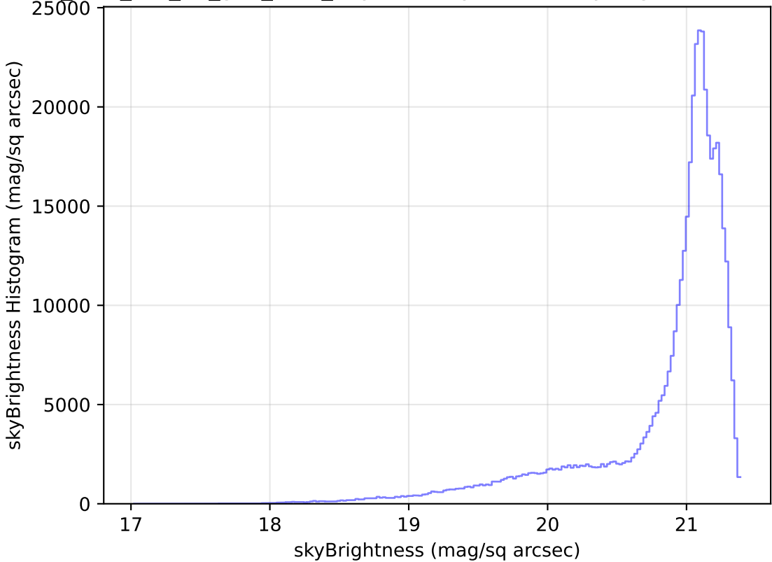
too_elab_r64_d2_griz_v3.4_10yrs All sky r band: skyBrightness Histogram
