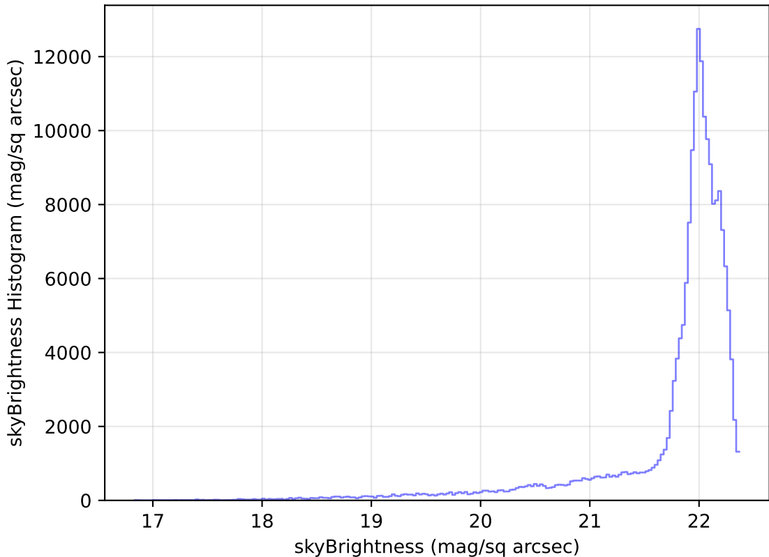
too_elab_r64_d2_griz_v3.4_10yrs All sky g band: skyBrightness Histogram
