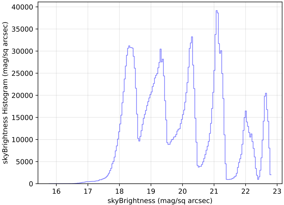
too_elab_r64_d2_griz_v3.4_10yrs All sky all bands: skyBrightness Histogram
