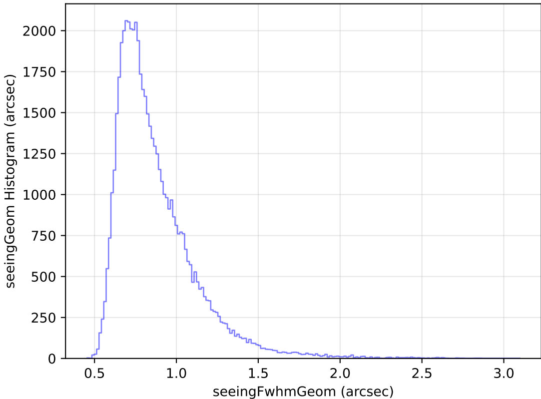
too_elab_r64_d2_griz_v3.4_10yrs Yr 1 i band: seeingGeom Histogram
