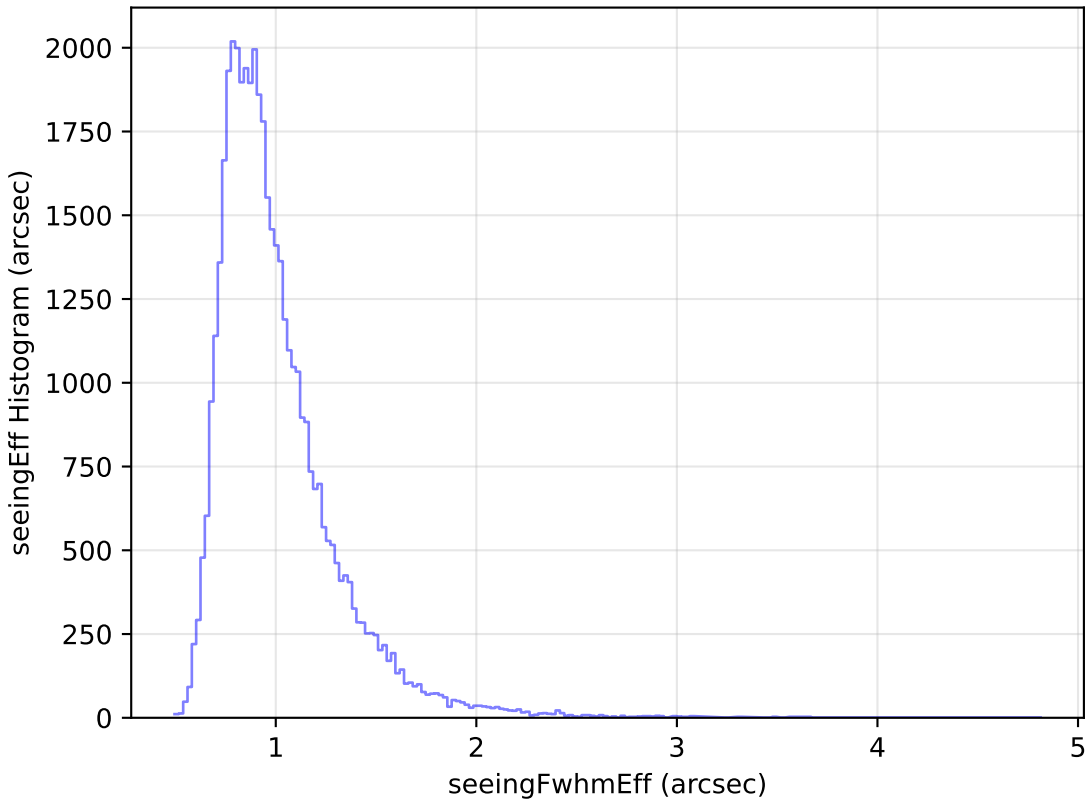
too_elab_r64_d2_griz_v3.4_10yrs Yr 1 z band: seeingEff Histogram
