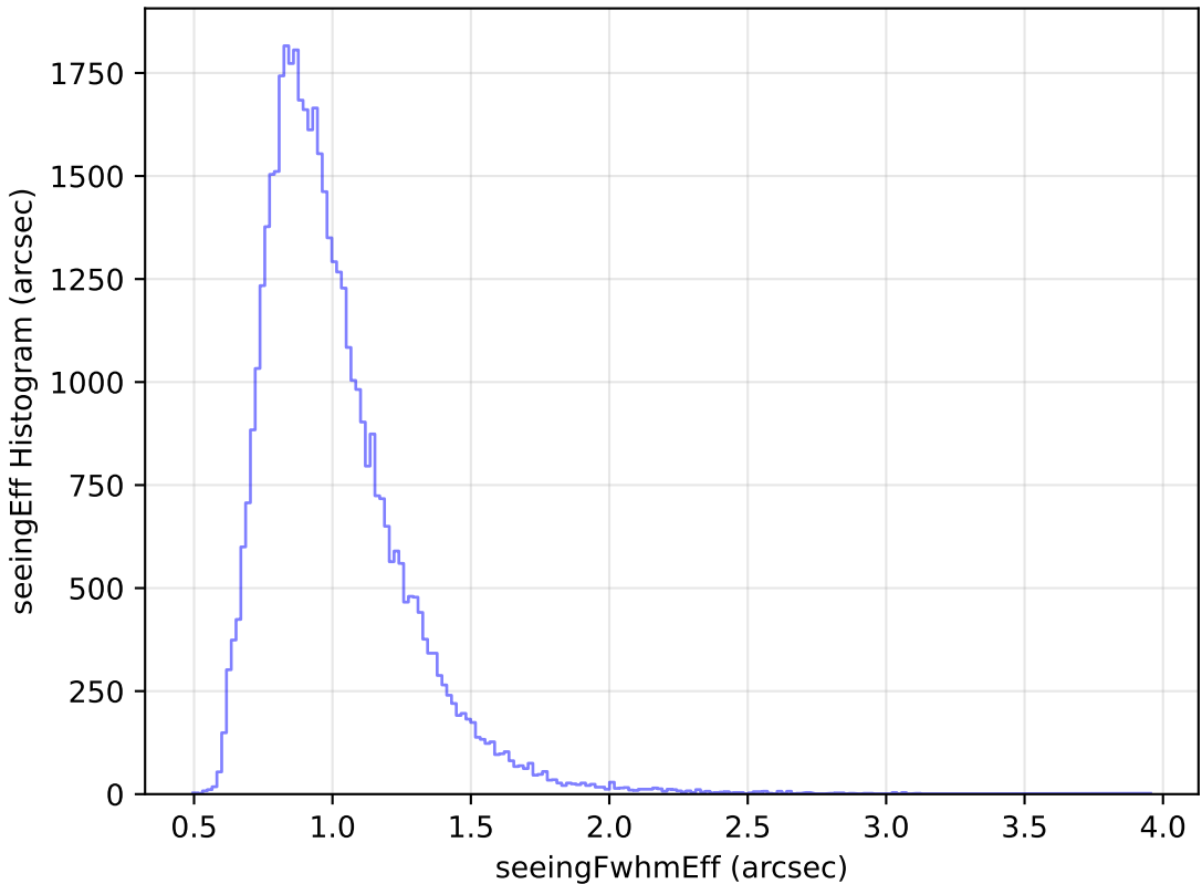
too_elab_r64_d2_griz_v3.4_10yrs Yr 1 y band: seeingEff Histogram
