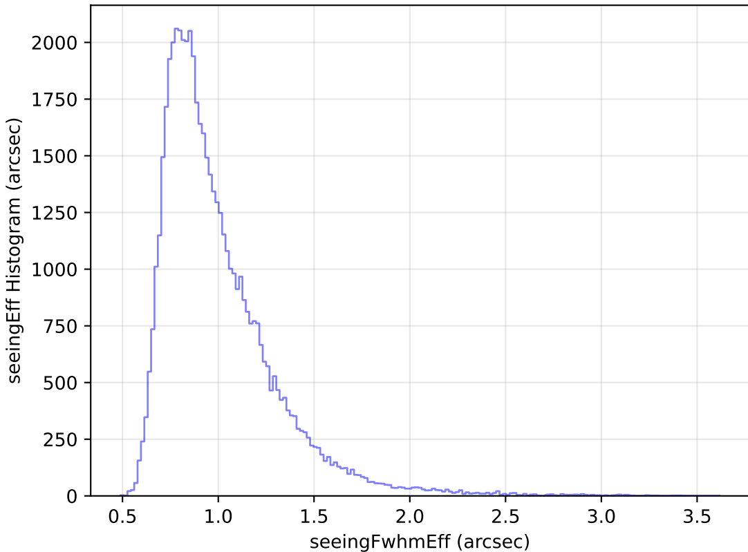
too_elab_r64_d2_griz_v3.4_10yrs Yr 1 i band: seeingEff Histogram
