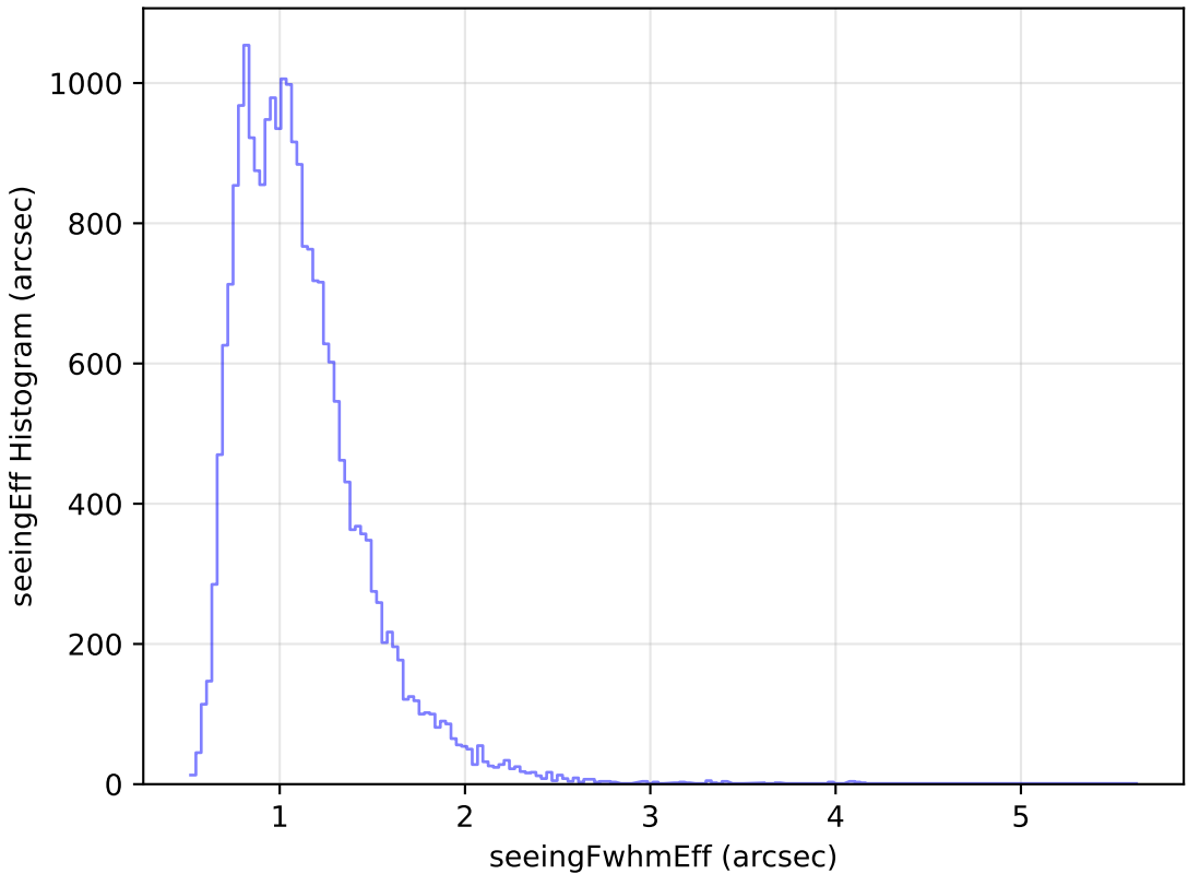
too_elab_r64_d2_griz_v3.4_10yrs Yr 1 g band: seeingEff Histogram
