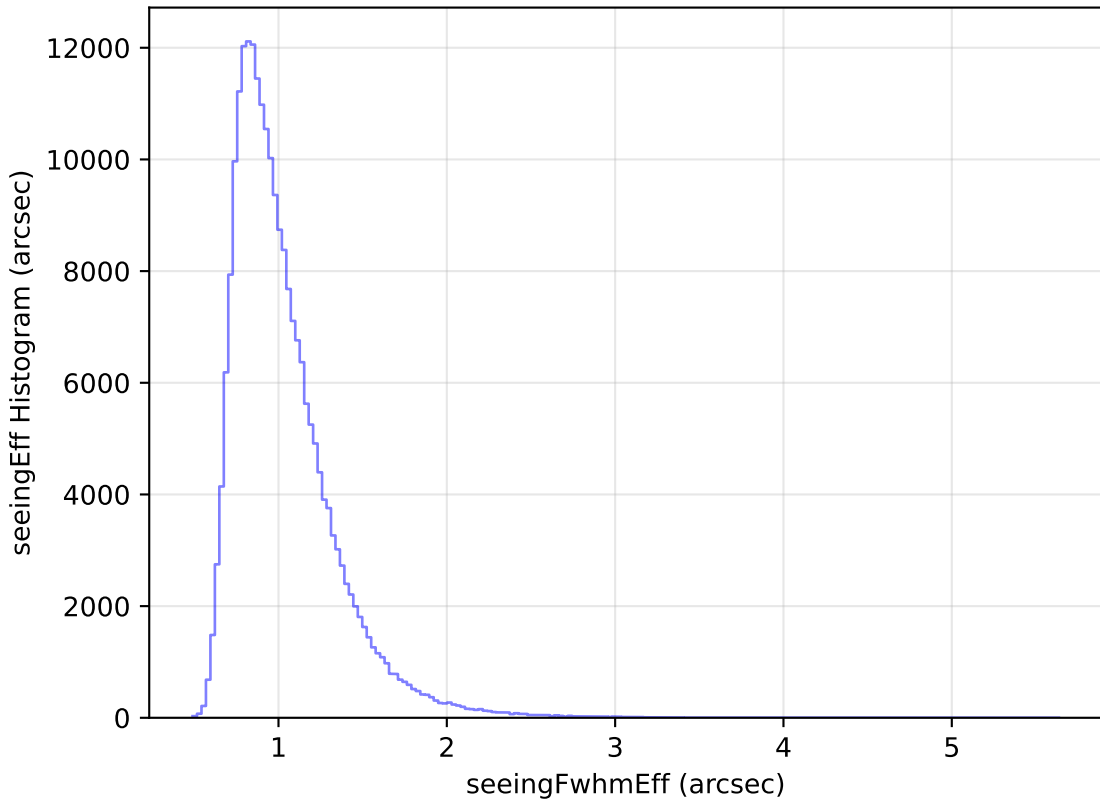
too_elab_r64_d2_griz_v3.4_10yrs Yr 1 all bands: seeingEff Histogram
