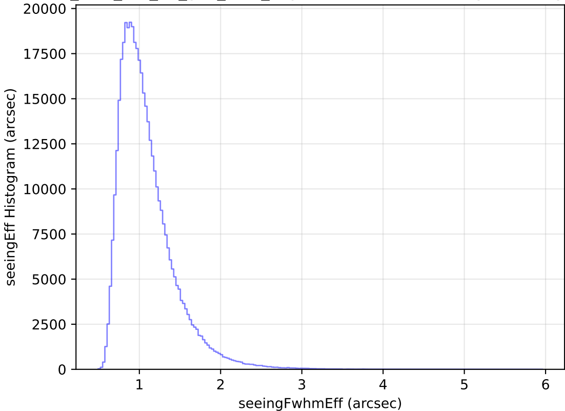
too_elab_r64_d2_griz_v3.4_10yrs WFD z band: seeingEff Histogram
