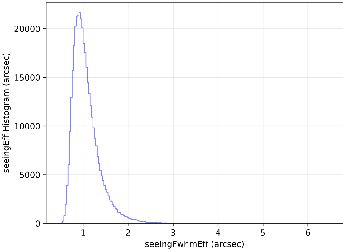
too_elab_r64_d2_griz_v3.4_10yrs WFD y band: seeingEff Histogram
