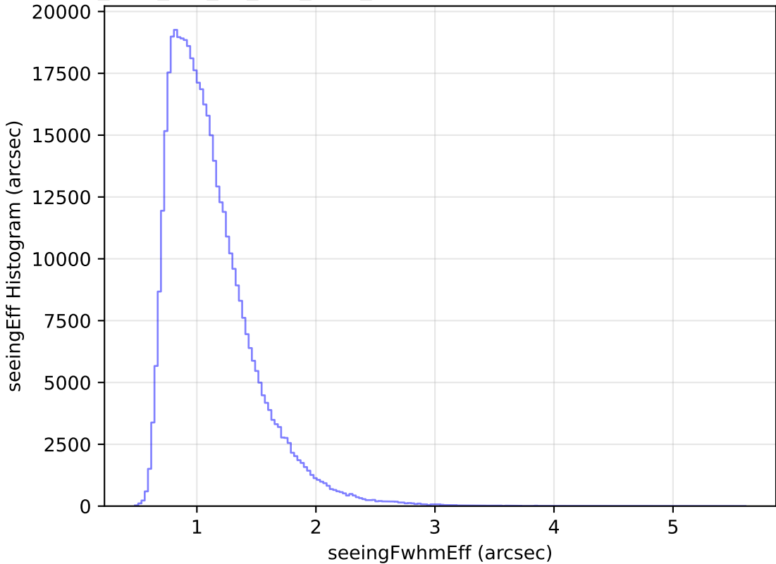
too_elab_r64_d2_griz_v3.4_10yrs WFD r band: seeingEff Histogram
