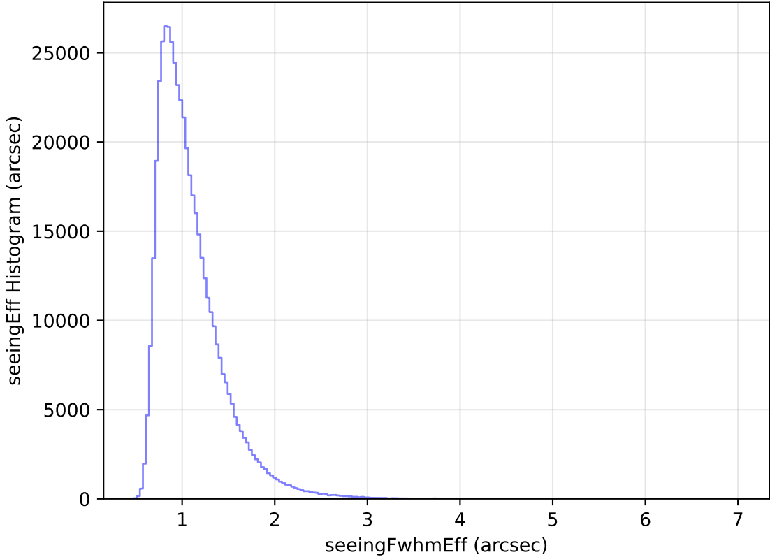
too_elab_r64_d2_griz_v3.4_10yrs WFD i band: seeingEff Histogram
