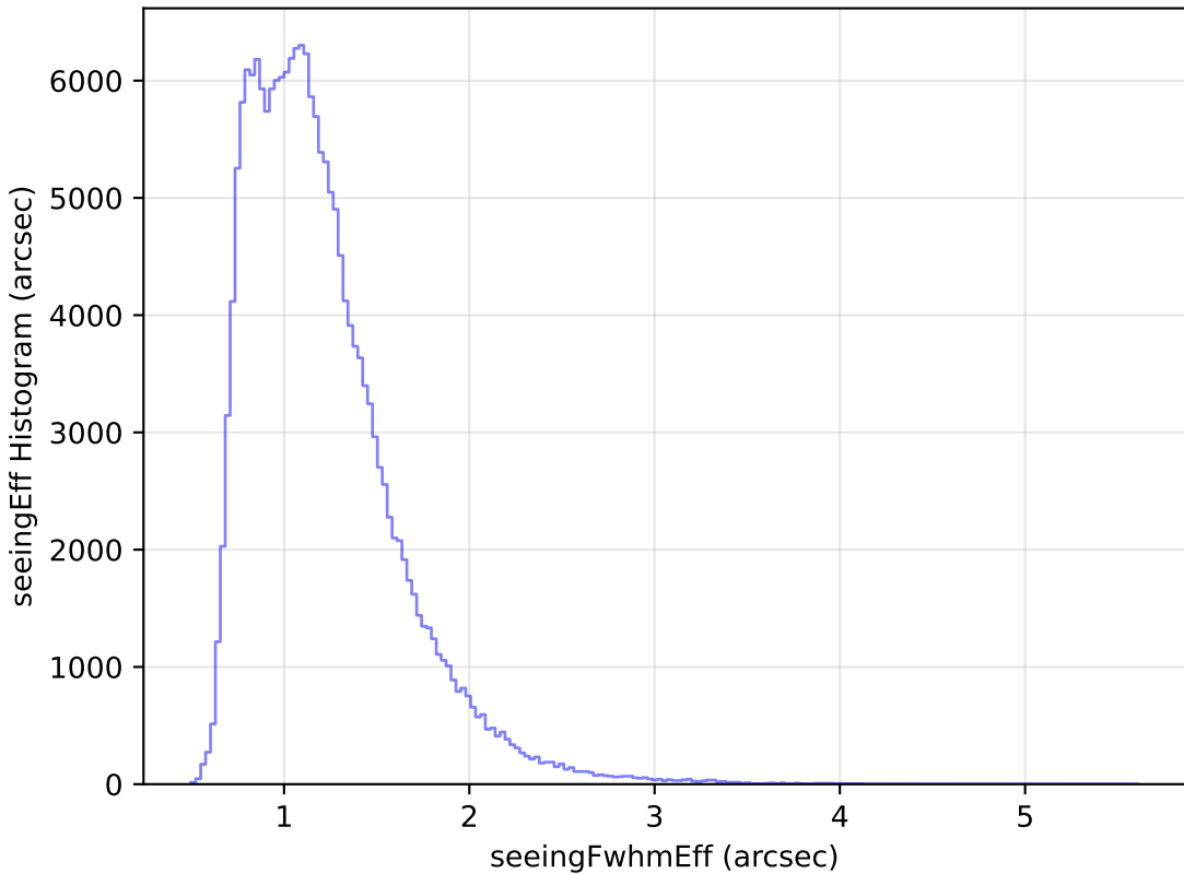
too_elab_r64_d2_griz_v3.4_10yrs WFD g band: seeingEff Histogram
