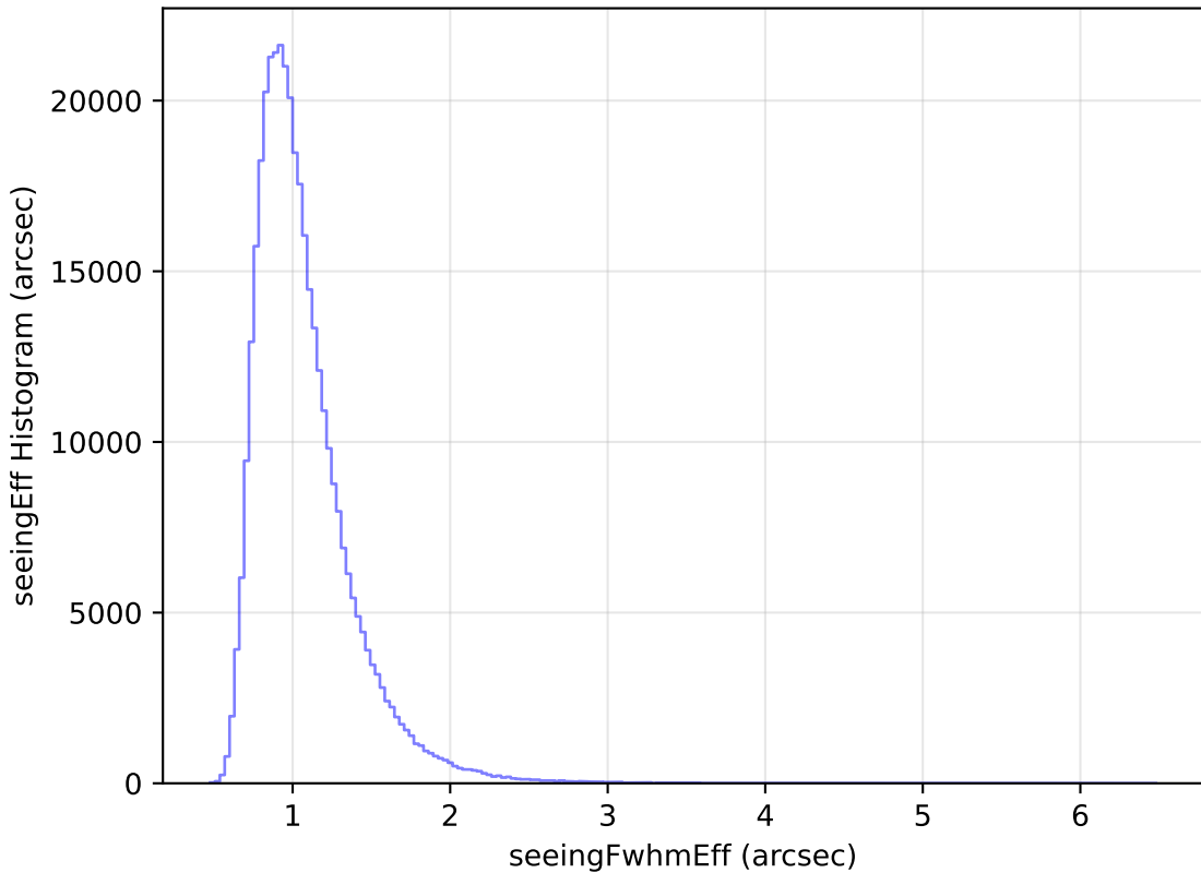
too_elab_r64_d2_griz_v3.4_10yrs All sky y band: seeingEff Histogram
