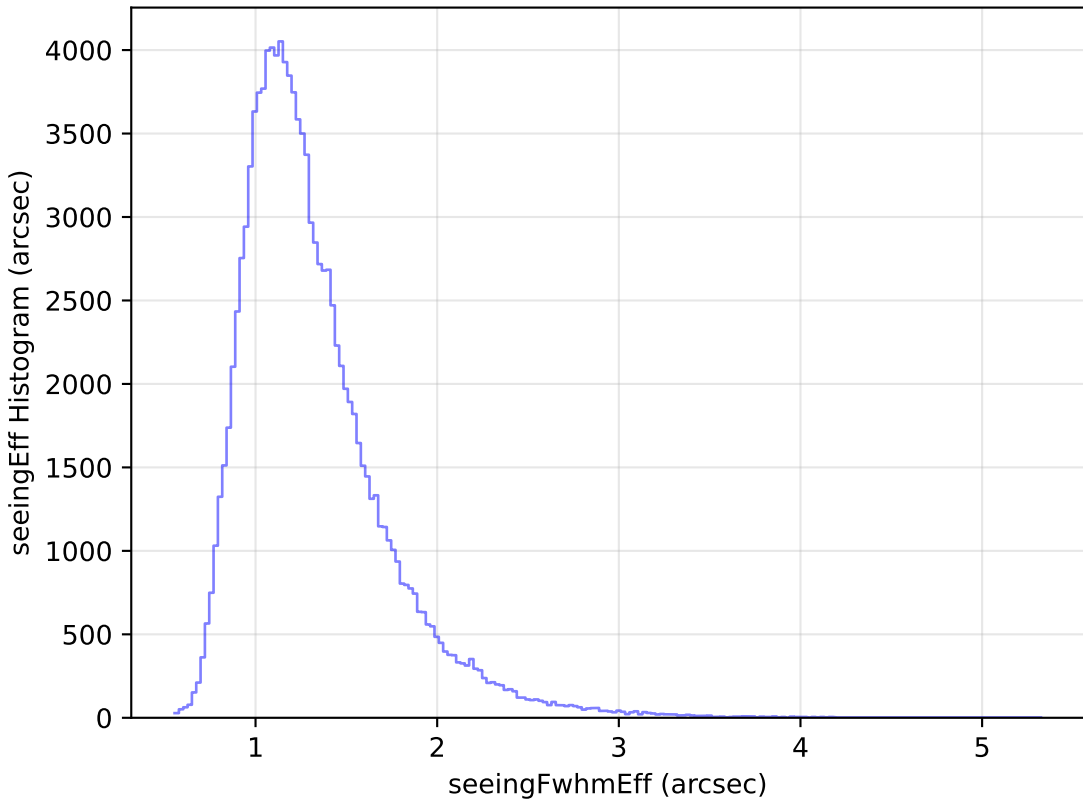
too_elab_r64_d2_griz_v3.4_10yrs All sky u band: seeingEff Histogram
