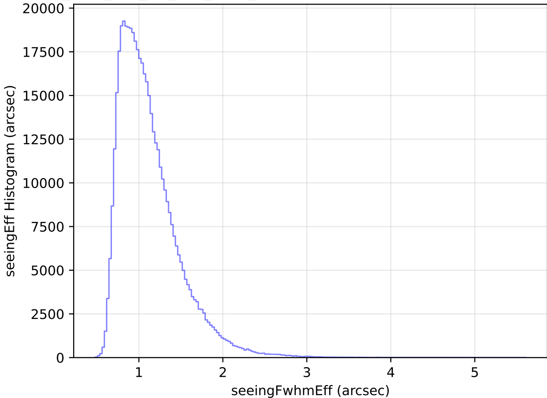
too_elab_r64_d2_griz_v3.4_10yrs All sky r band: seeingEff Histogram
