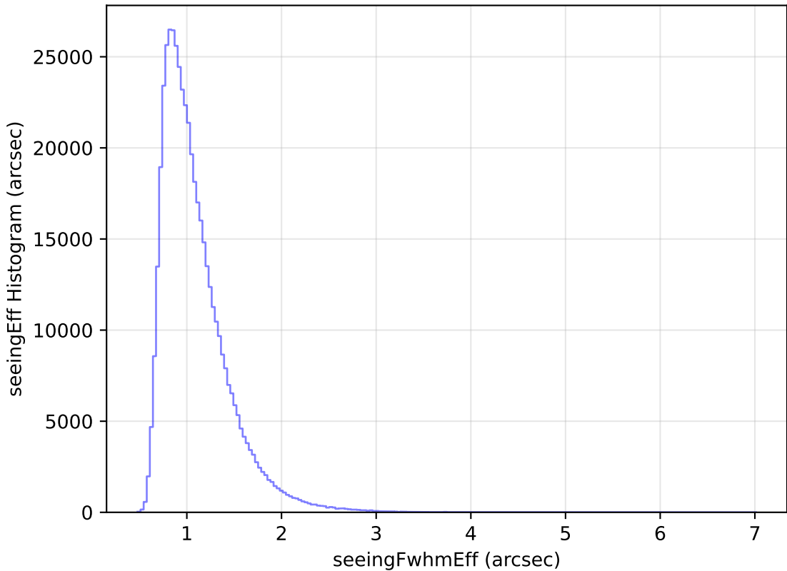
too_elab_r64_d2_griz_v3.4_10yrs All sky i band: seeingEff Histogram
