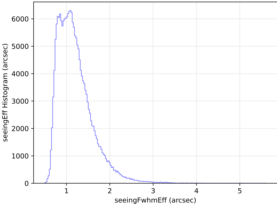
too_elab_r64_d2_griz_v3.4_10yrs All sky g band: seeingEff Histogram
