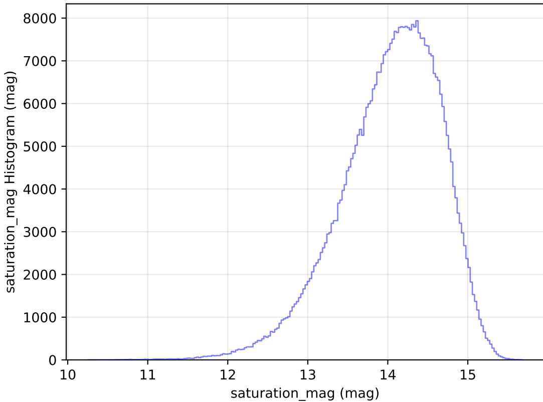
too_elab_r64_d2_griz_v3.4_10yrs WFD z band: saturation_mag Histogram
