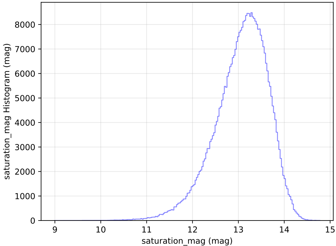
too_elab_r64_d2_griz_v3.4_10yrs WFD y band: saturation_mag Histogram
