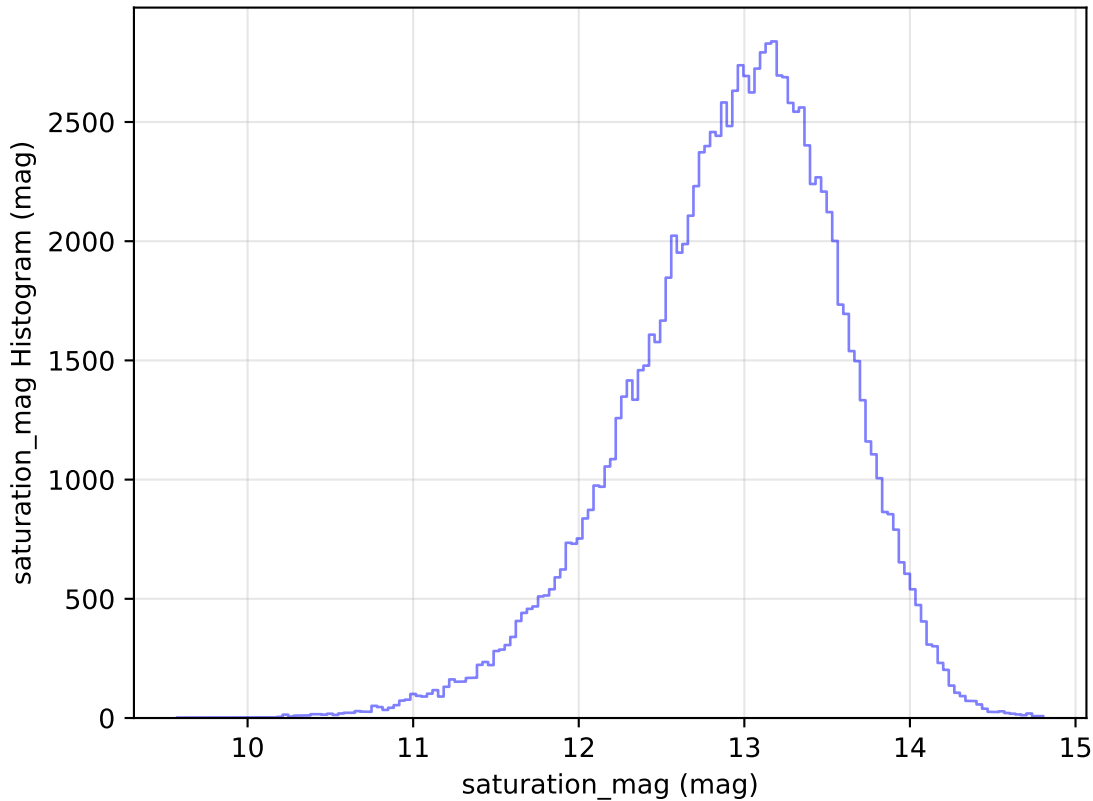
too_elab_r64_d2_griz_v3.4_10yrs WFD u band: saturation_mag Histogram
