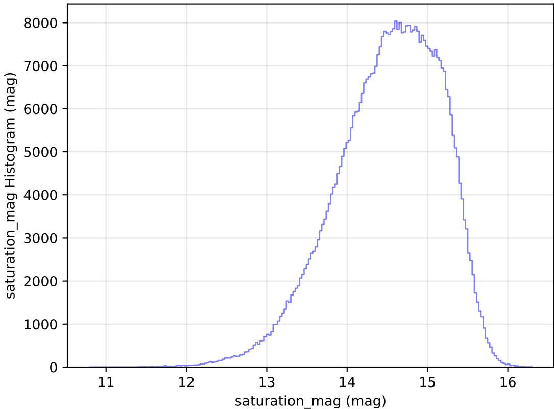
too_elab_r64_d2_griz_v3.4_10yrs WFD r band: saturation_mag Histogram
