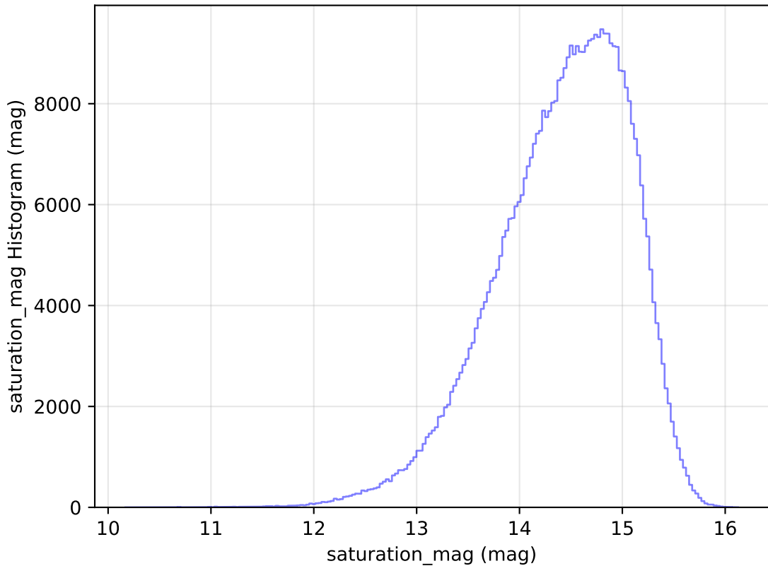
too_elab_r64_d2_griz_v3.4_10yrs WFD i band: saturation_mag Histogram
