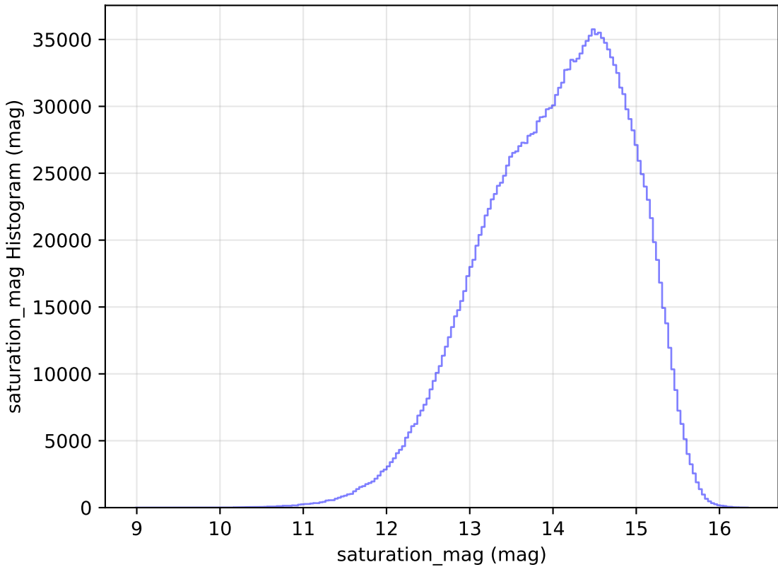
too_elab_r64_d2_griz_v3.4_10yrs WFD all bands: saturation_mag Histogram
