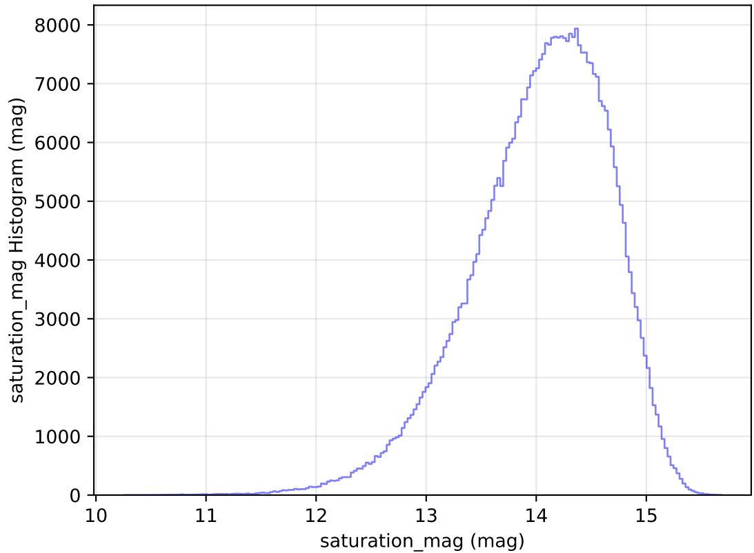
too_elab_r64_d2_griz_v3.4_10yrs All sky z band: saturation_mag Histogram
