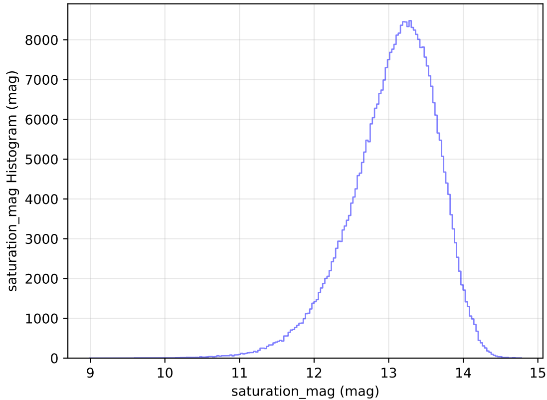
too_elab_r64_d2_griz_v3.4_10yrs All sky y band: saturation_mag Histogram
