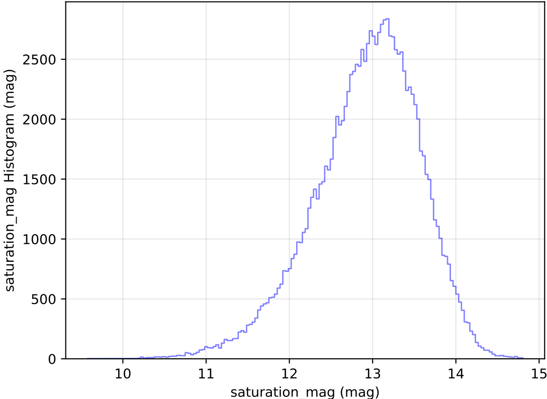
too_elab_r64_d2_griz_v3.4_10yrs All sky u band: saturation_mag Histogram
