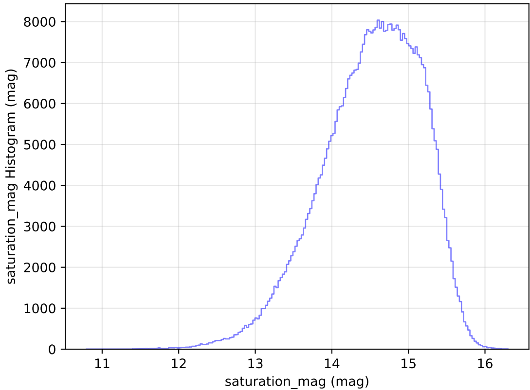
too_elab_r64_d2_griz_v3.4_10yrs All sky r band: saturation_mag Histogram
