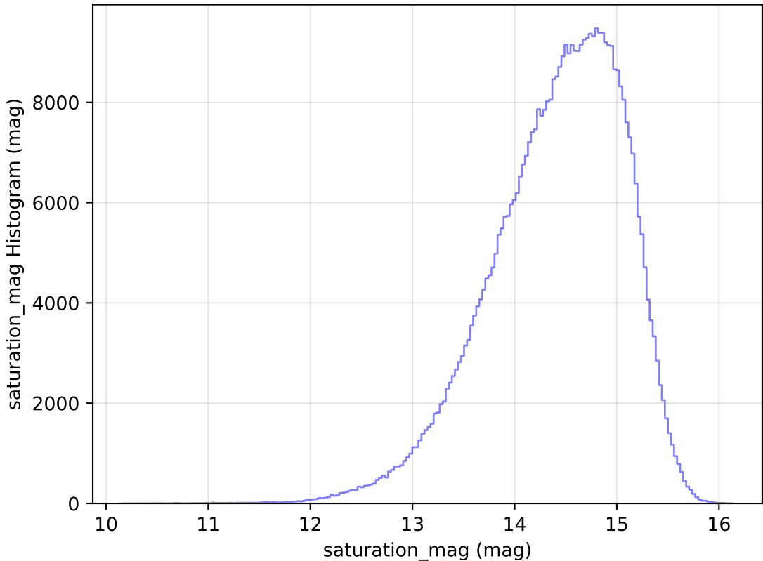
too_elab_r64_d2_griz_v3.4_10yrs All sky i band: saturation_mag Histogram
