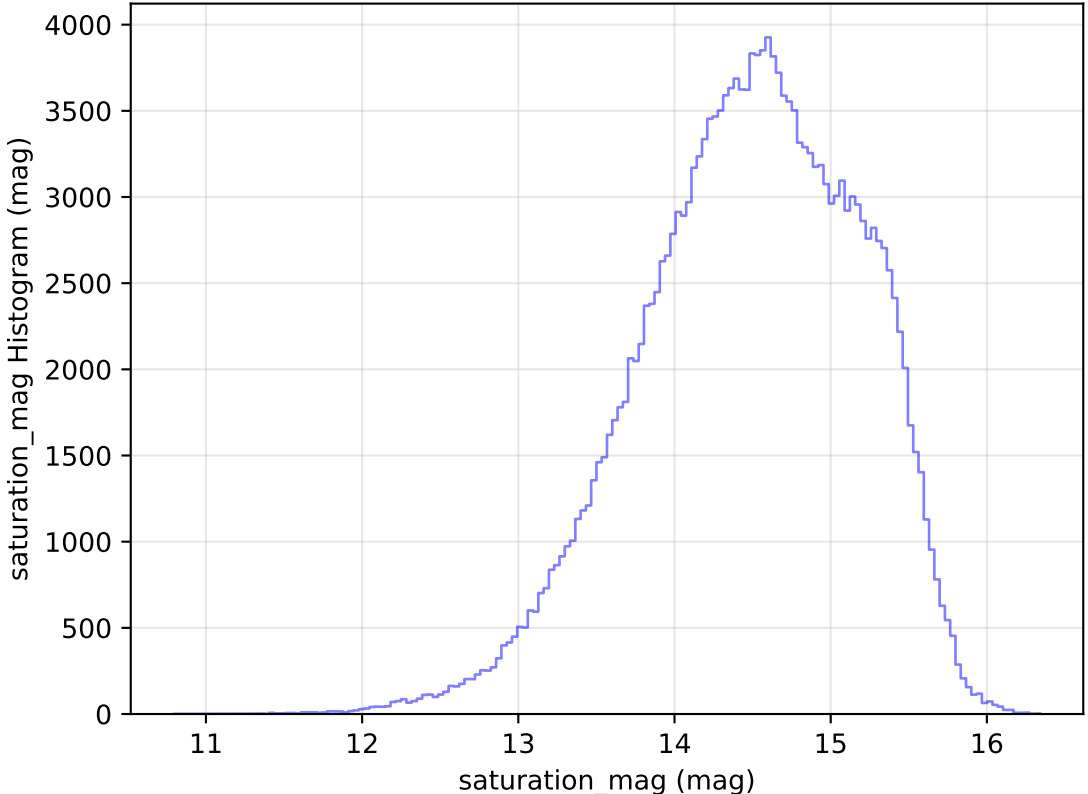
too_elab_r64_d2_griz_v3.4_10yrs All sky g band: saturation_mag Histogram
