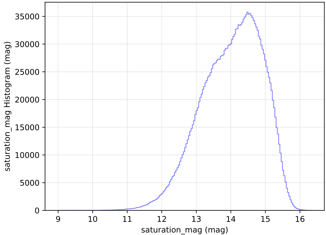
too_elab_r64_d2_griz_v3.4_10yrs All sky all bands: saturation_mag Histogram
