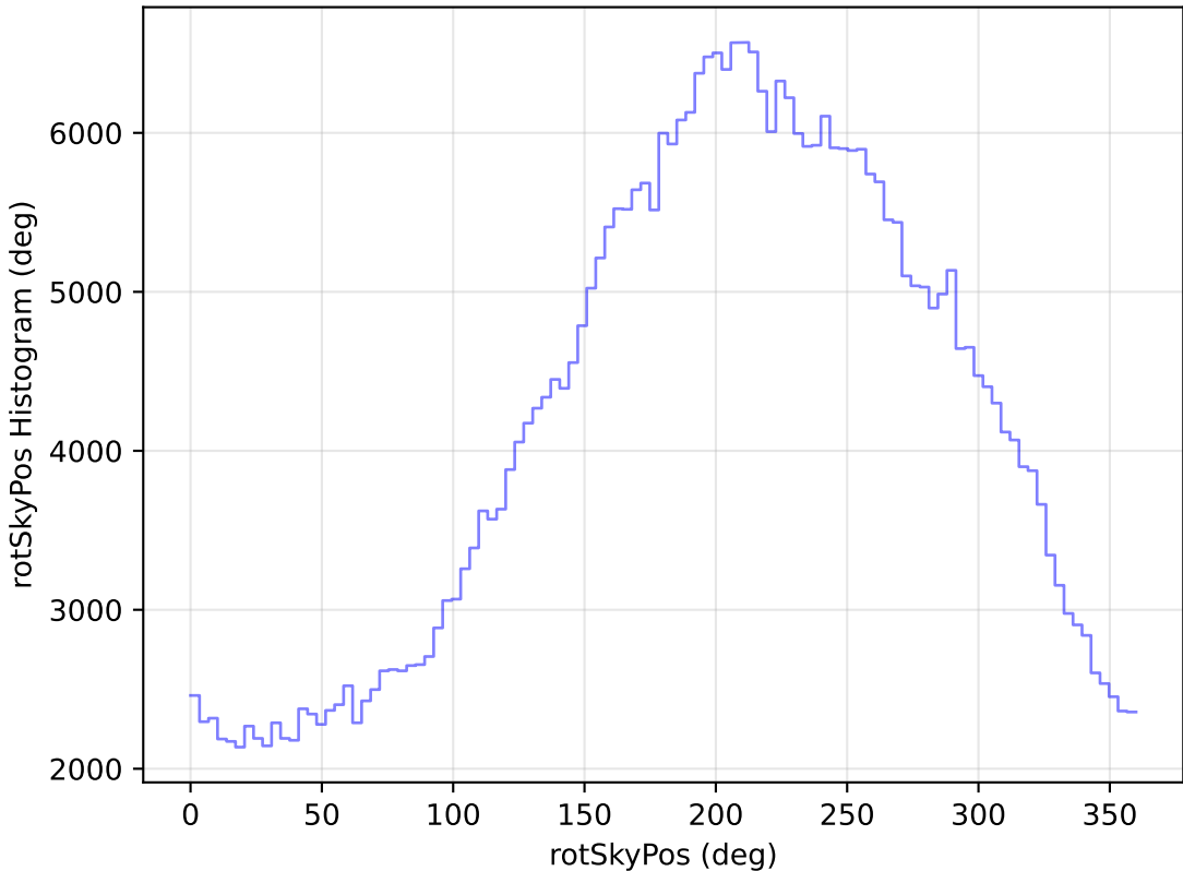
too_elab_r64_d2_griz_v3.4_10yrs WFD z band: rotSkyPos Histogram
