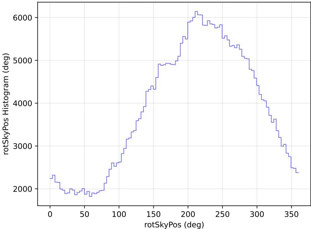
too_elab_r64_d2_griz_v3.4_10yrs WFD y band: rotSkyPos Histogram
