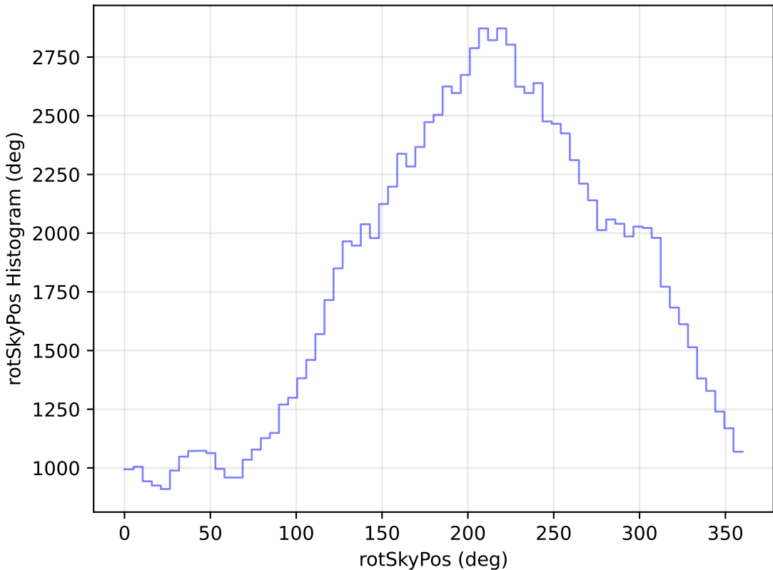
too_elab_r64_d2_griz_v3.4_10yrs WFD u band: rotSkyPos Histogram
