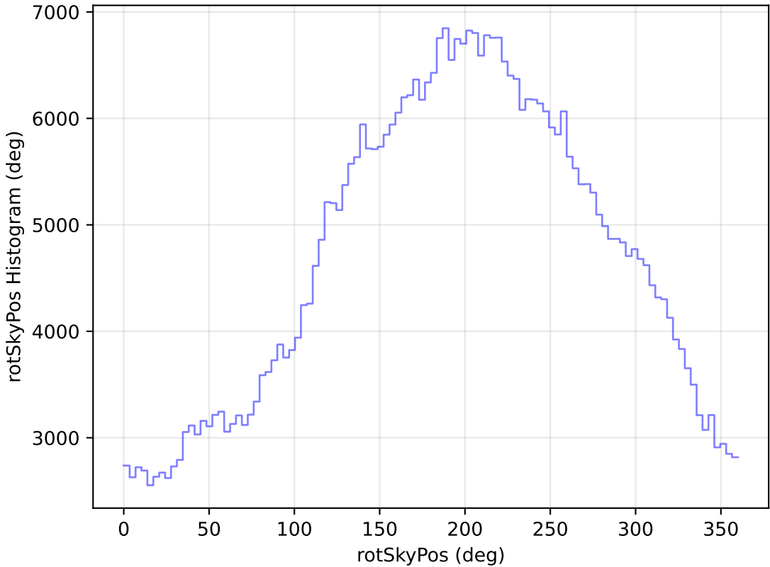
too_elab_r64_d2_griz_v3.4_10yrs WFD r band: rotSkyPos Histogram
