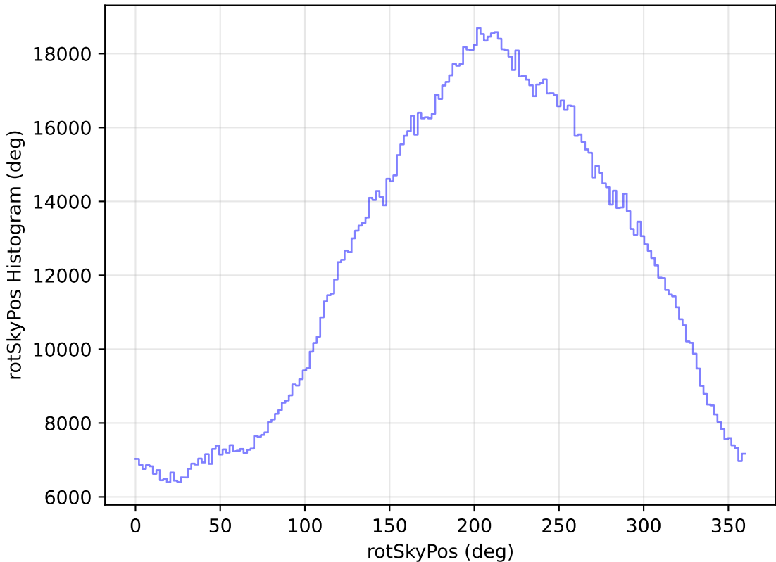
too_elab_r64_d2_griz_v3.4_10yrs WFD all bands: rotSkyPos Histogram
