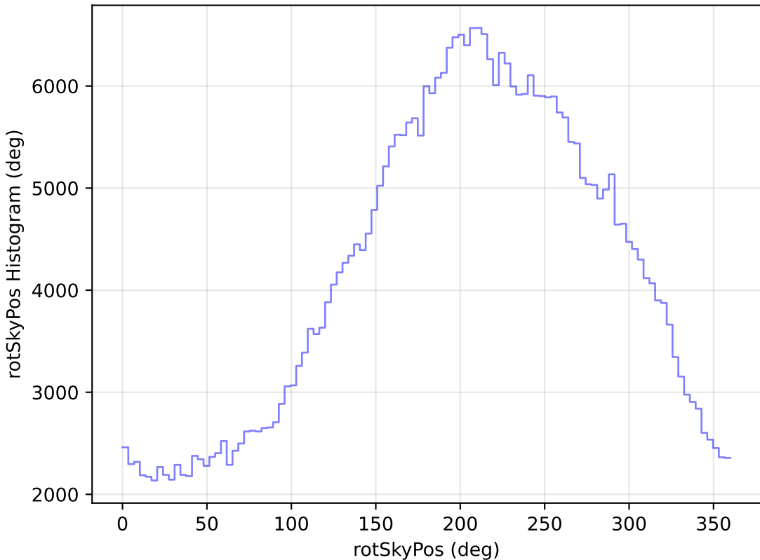
too_elab_r64_d2_griz_v3.4_10yrs All sky z band: rotSkyPos Histogram
