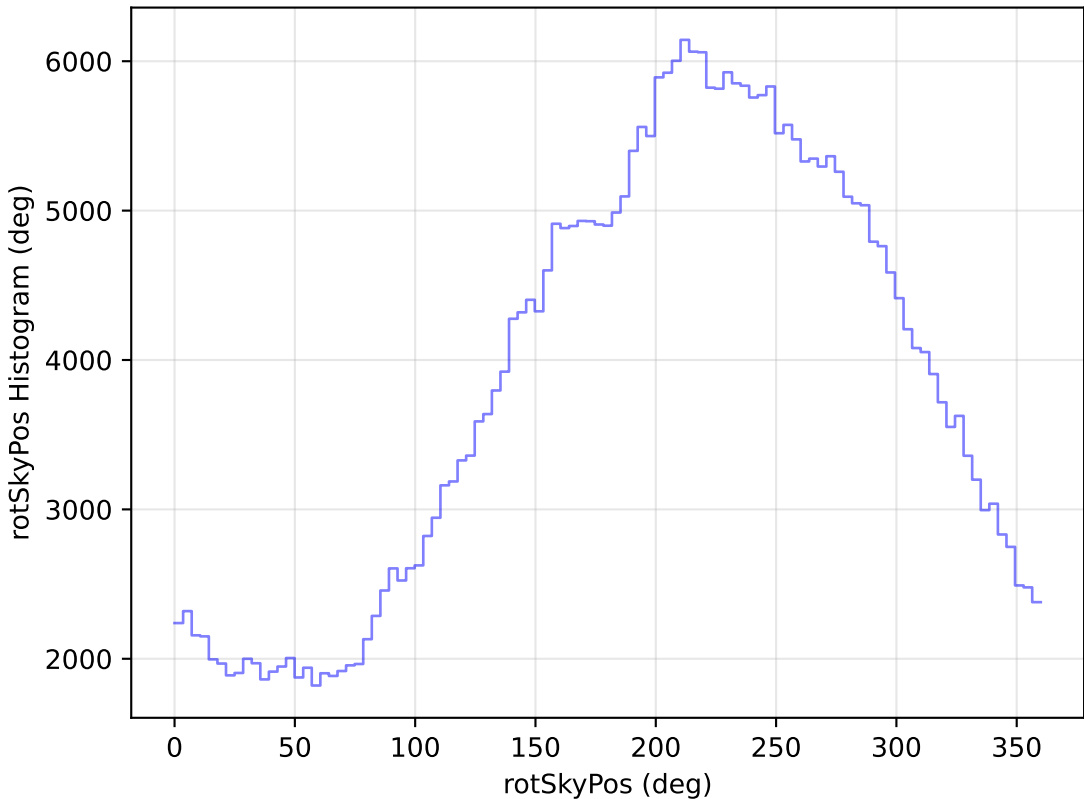
too_elab_r64_d2_griz_v3.4_10yrs All sky y band: rotSkyPos Histogram
